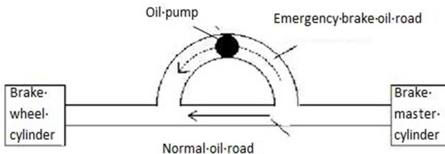
Figure 1. Hydraulic auxiliary brake device.
